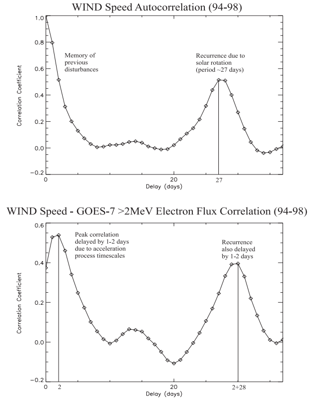
Figure 3: Linear Analysis of Solar Wind Speed Data
