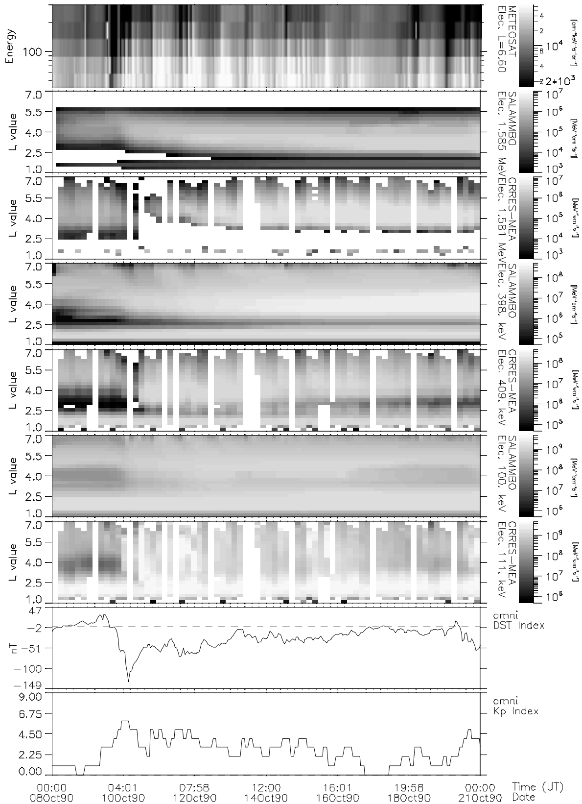
Plate2. Comparison between measurements and simulation for the October 8-October 21, 1990 period: Kp and Dst (first and 2 nd panels from the bottom), CRRES-MEA and Salammbô for nearly 100 keV (3 rd and 4 th panels), for around 400 keV (5 th and 6 th panels), and for around 1600 keV (7 th and 8 th panels), and Meteosat-3 measurements (9 th panel, at the top), used as boundary conditions for the simulation.
