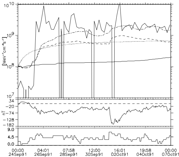
Figure 1. The September 24, 1991 storm: K_p (lower panel), Dst (middle panel), around 100 keV omnidirectional fluxes in the L = 4 region from CRRES-MEA (noisy solid curve), from Salammbô using standard (solid line), 5 times standard (dotted line), K_p dependent (dotted and dot-dashed lines) radial diffusion coefficients, the dot-dashed line being also with a K_p dependent plasmopause location.
