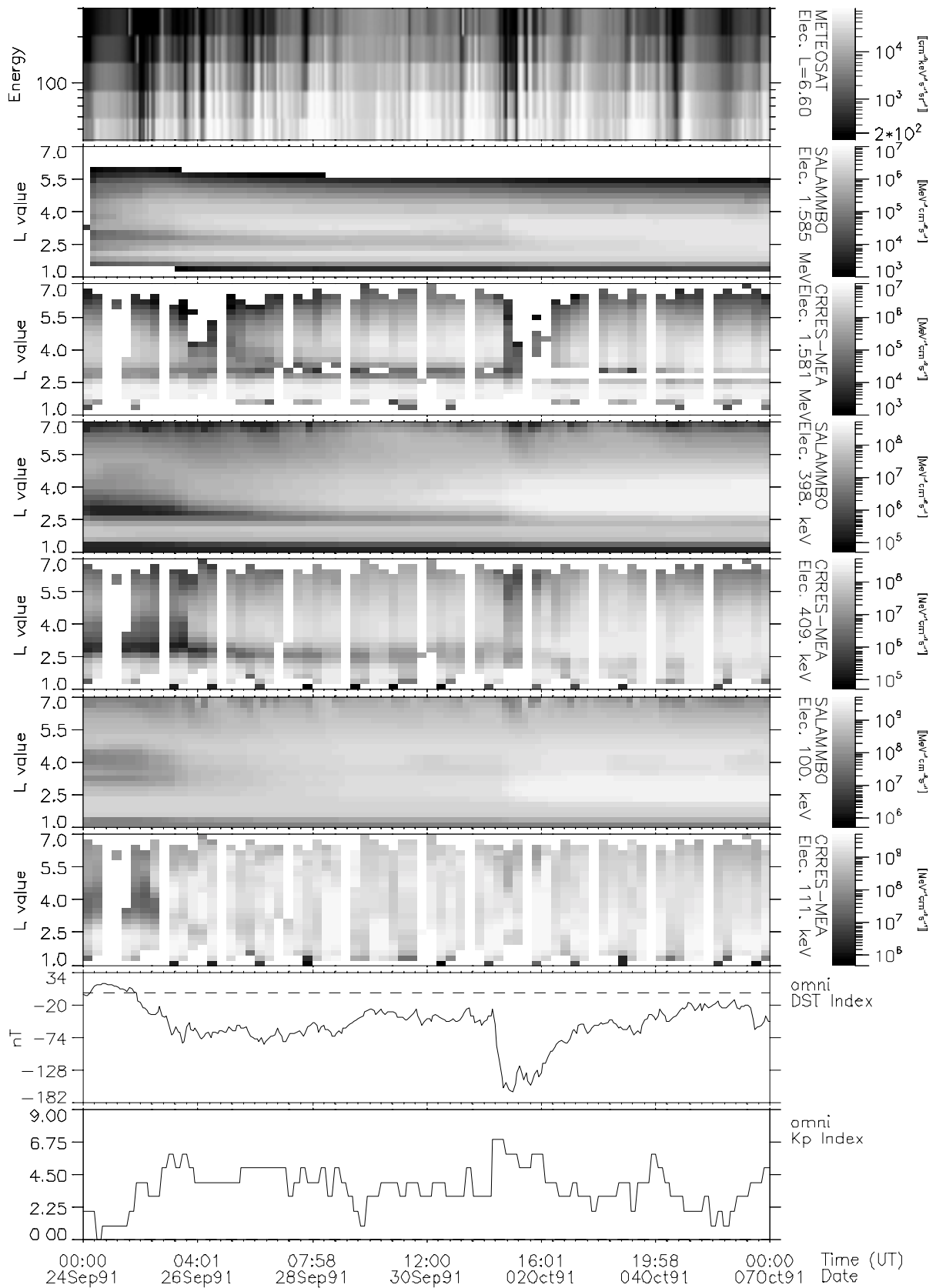
Plate1. Comparison between measurements and simulation for the September 24-October 7, 1991 period: Kp and Dst (first and 2 nd panels from the bottom), CRRES-MEA and Salammbô for nearly 100 keV (3 rd and 4 th panels), for around 400 keV (5 th and 6 th panels), and for around 1600 keV (7 th and 8 th panels), and Meteosat-3 measurements (9 th panel, at the top), used as boundary conditions for the simulation.
