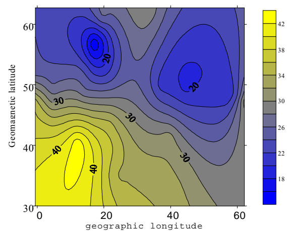
Figure 4.b The distribution of mean critical electron density( \text{MHz} \cdot 10 ) for four very disturb days with K_p > 4+ , over COST 251 area, covered the ARIEL 4 time domain, constructed by use the ionosonde ground based measurements.
